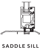
SADDLE SILL
