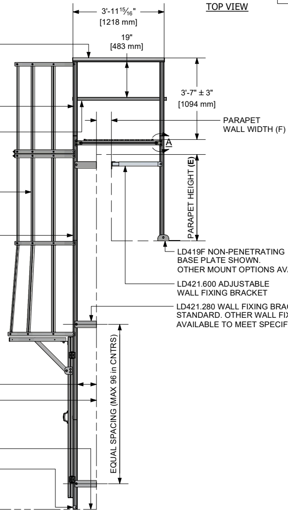
SIDE VIEW
