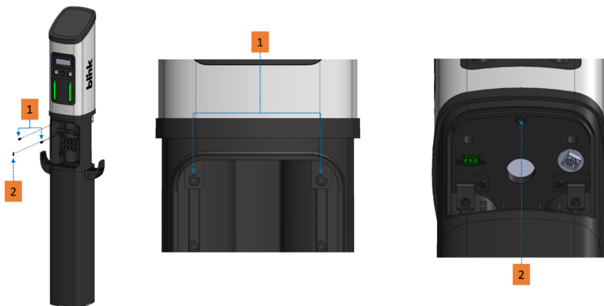
Fig. 24 – Head unit mounting screw locations
