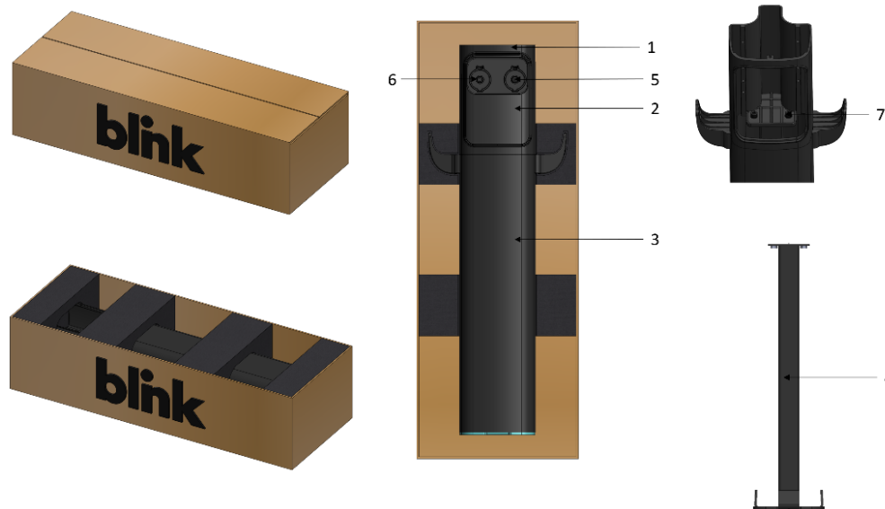
Fig. 13 – Pedestal components
