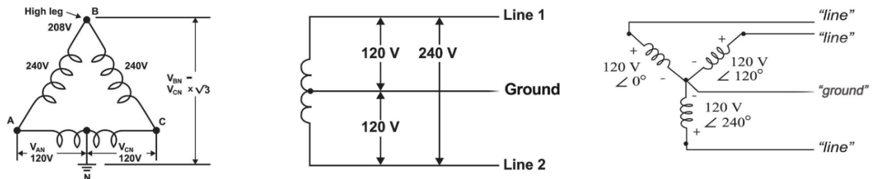
Fig. 9 – Acceptable transformer configurations
