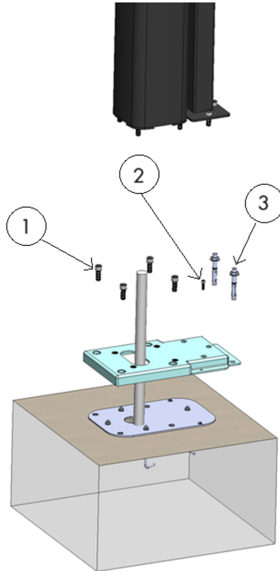
Fig. B-1 – Attaching Retrofit Adapter Plate to existing anchor plate
