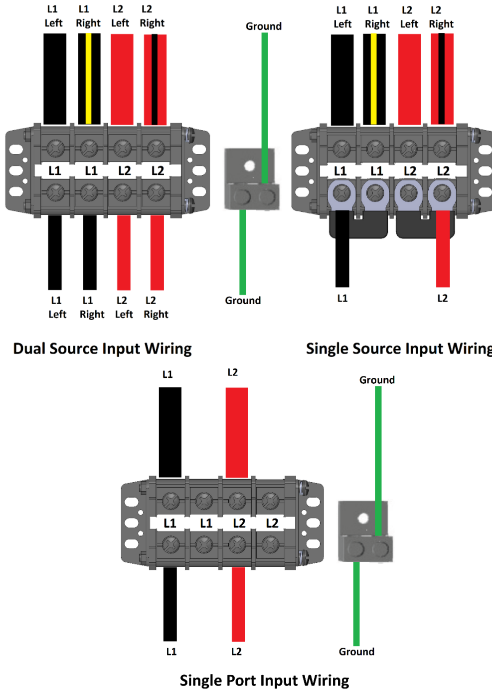
Fig. 11 – AC input connection diagrams
