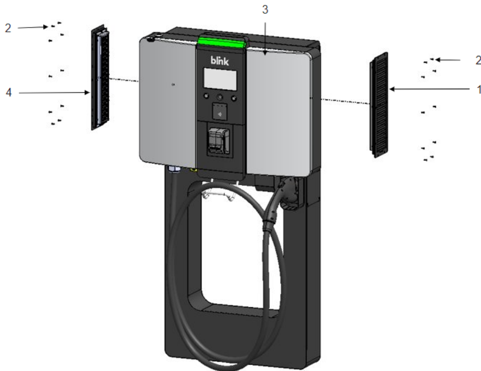
Fig. 62 – Air vent assemblies
