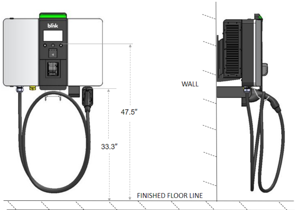
Fig. 45 – Charger with Wall Mount Dimensions
