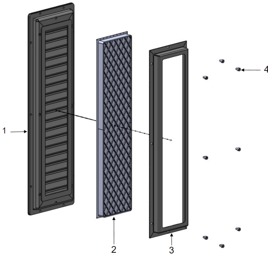
Fig. 63 – Air filter assembly
