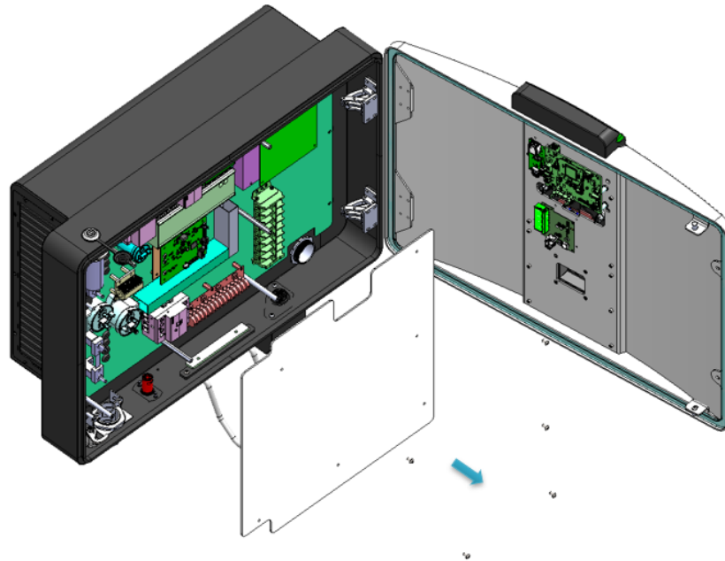
Fig. 48 – Remove plexiglass shield
