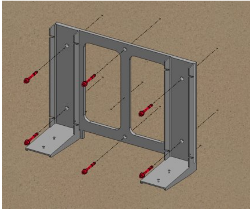
Fig. 36 – Wall mount anchor bolts
