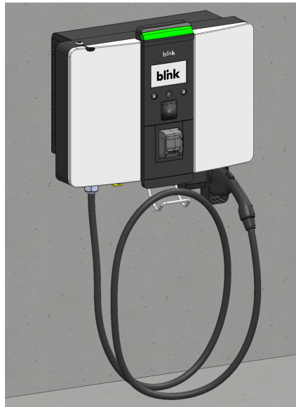
Fig. 46 – Final Assembly with Wall Mount
