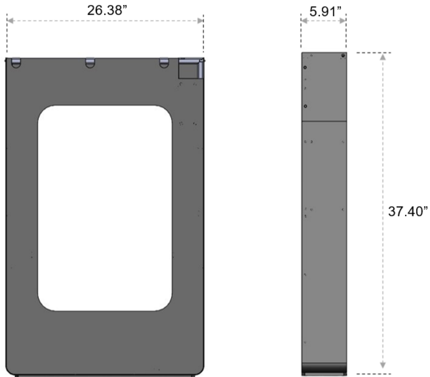
Fig. 4 – Pedestal Dimensions
