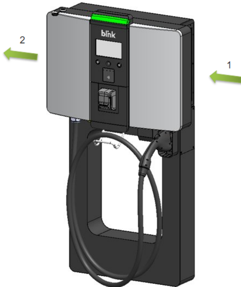
Fig. 6 – Direction of Ventilation Airflow
