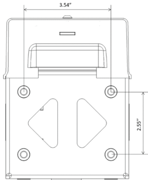
Fig. 19 – Cable management system wall mount bracket template
