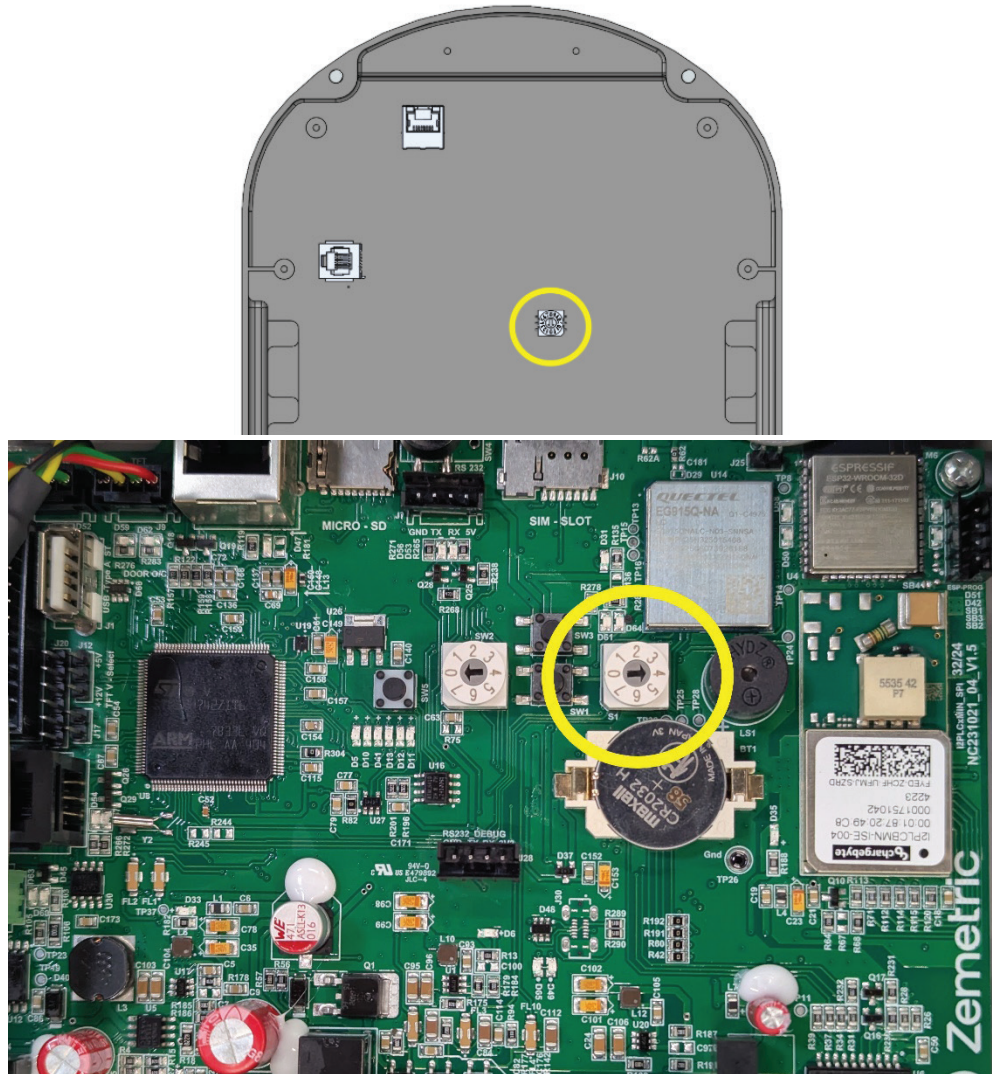
Fig. 17 – Derate switch location (labelled S1)
