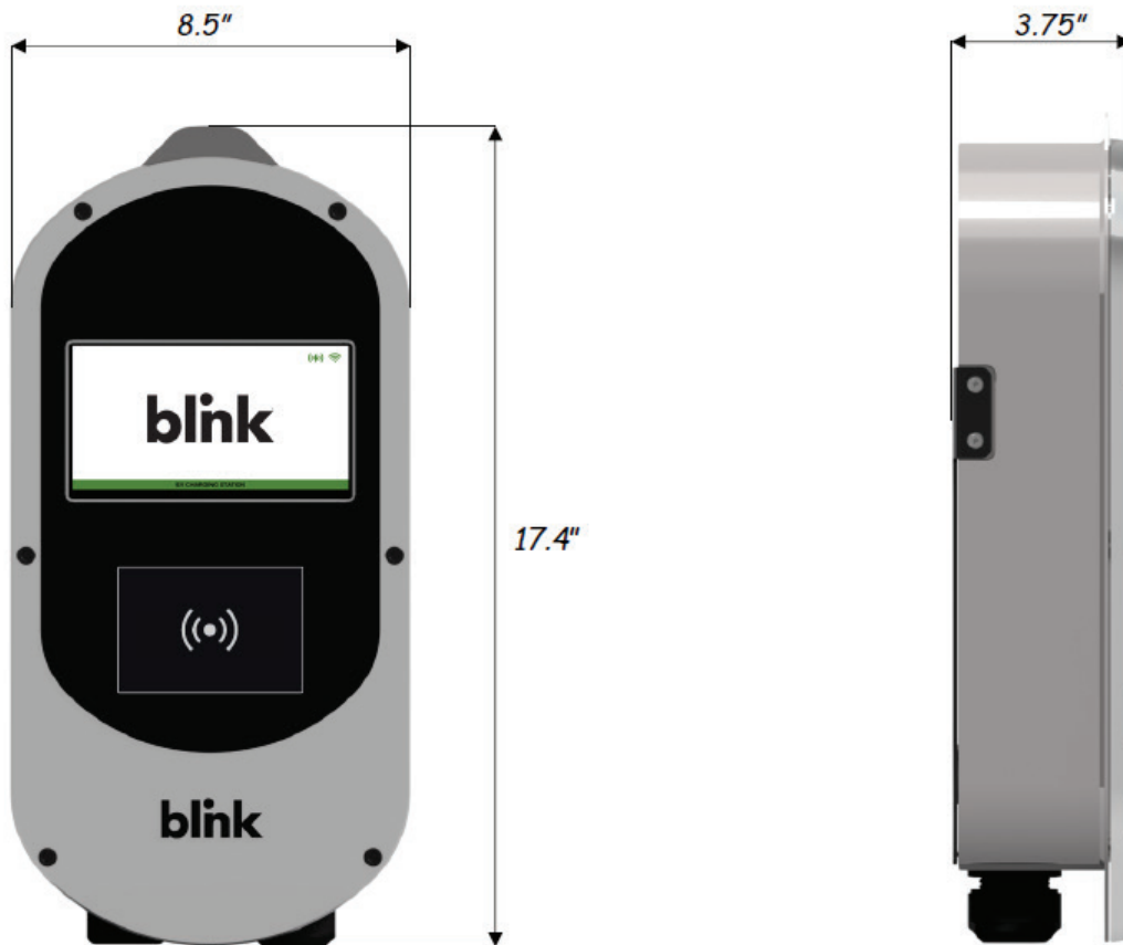
Fig. 1 – Shasta 48/80 charger
