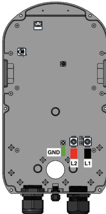
Fig. 14 – AC input wire connections
