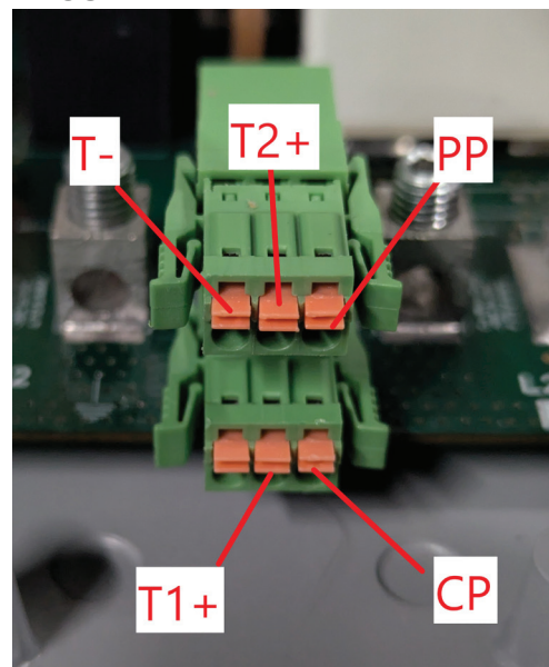
Fig. 16 – Output cable low-voltage connections
