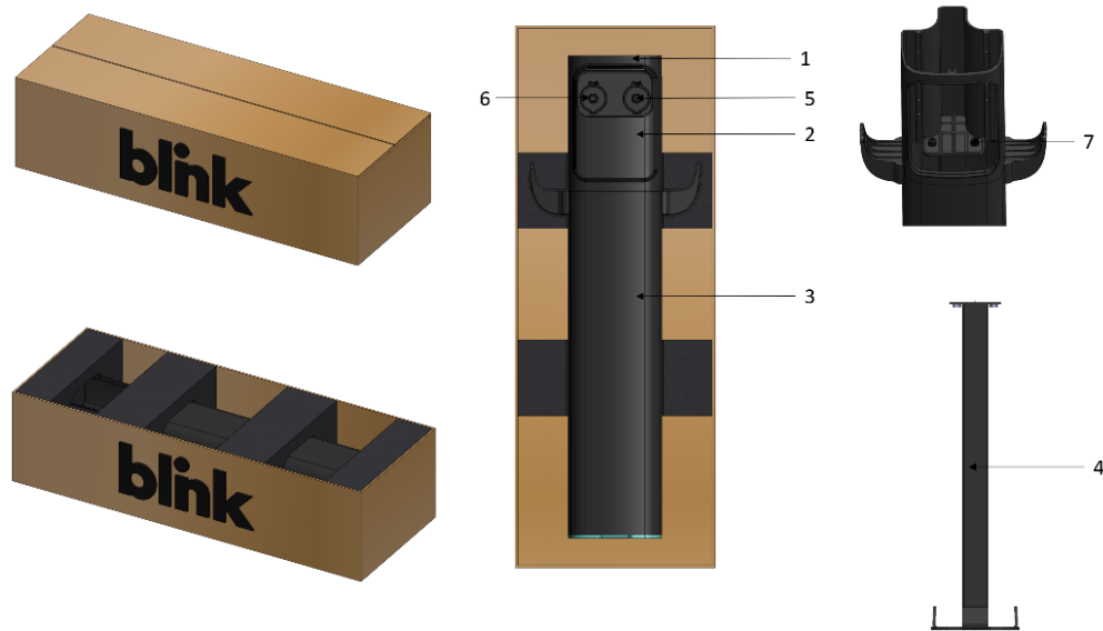
Fig. 13 – Pedestal components
