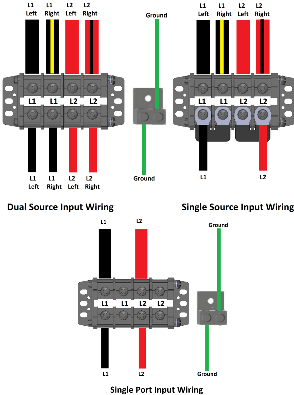
Fig. 11 – AC input connection diagrams
