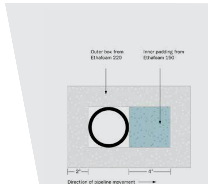
Figure 12 : T.E.B. cross section detail for 1" (25mm) of thermal expansion
